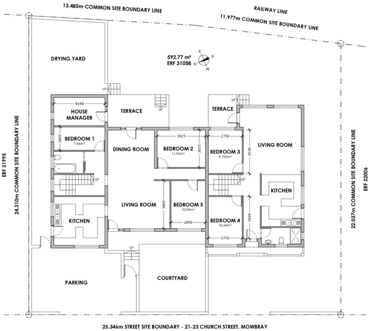
GROUND FLOOR LEVEL PLAN - 1:100
