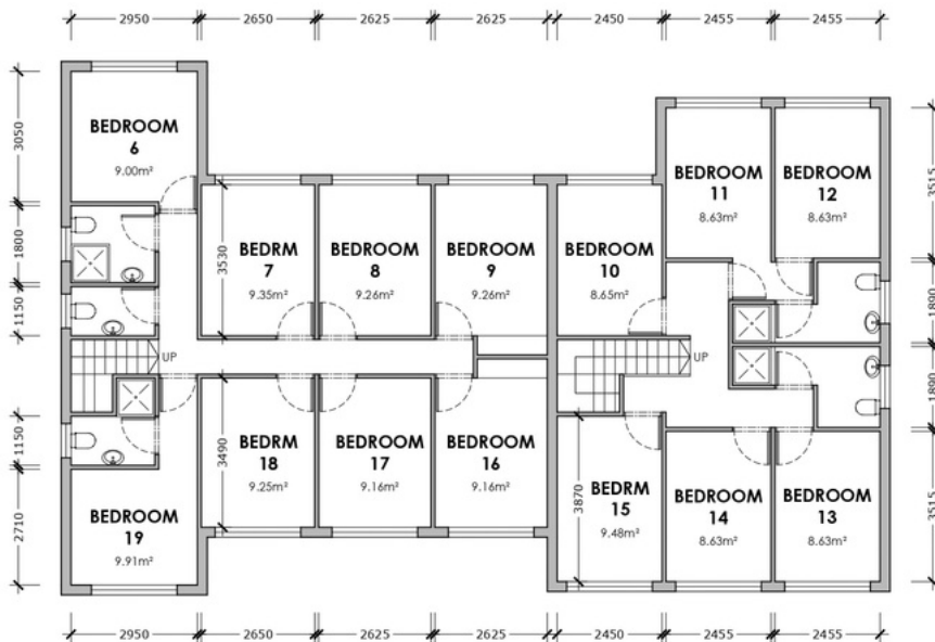
FIRST FLOOR LEVEL PLAN - 1:100
